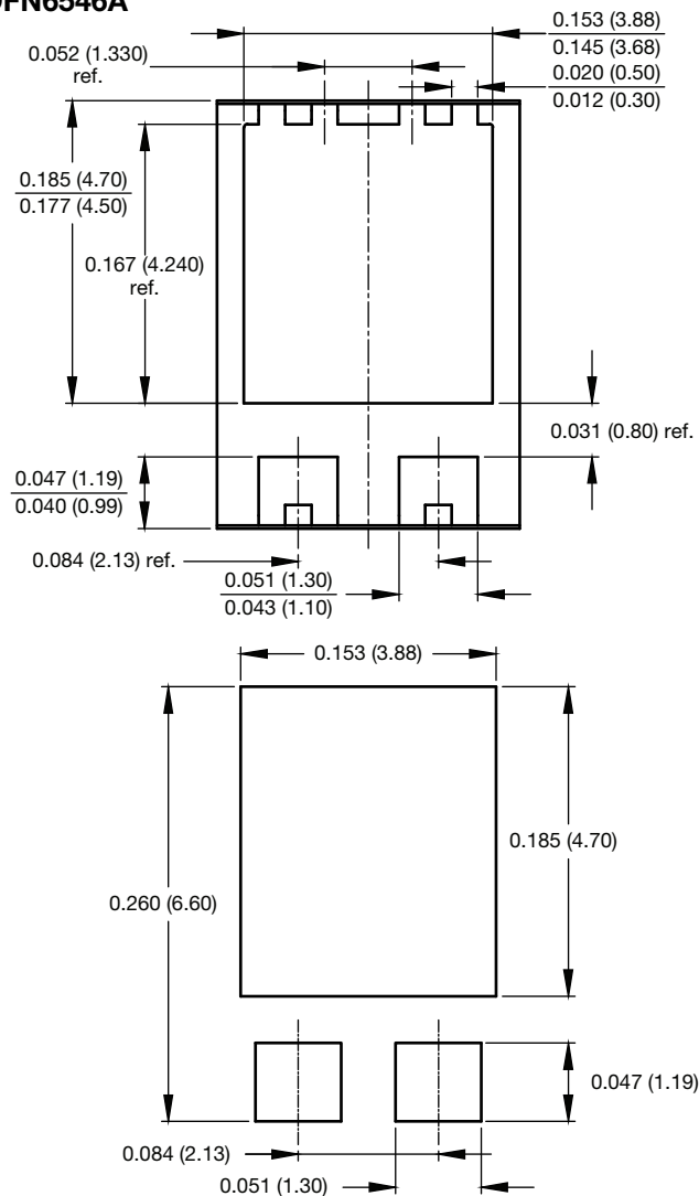
DFN6546A
