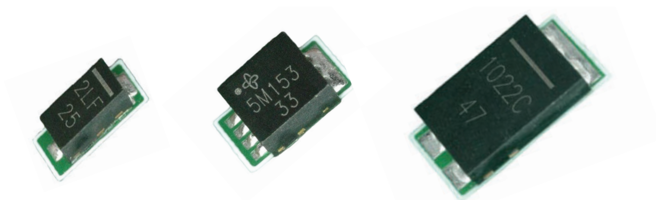
Real picture of DFN3820A, DFN33A, and DFN6546A after reflow soldering showing meniscus
