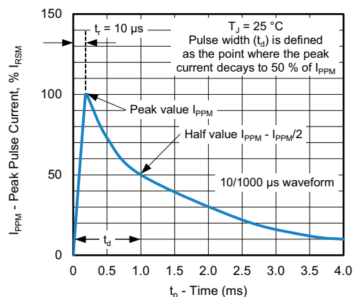
Fig. 10 - Pulse Waveform
