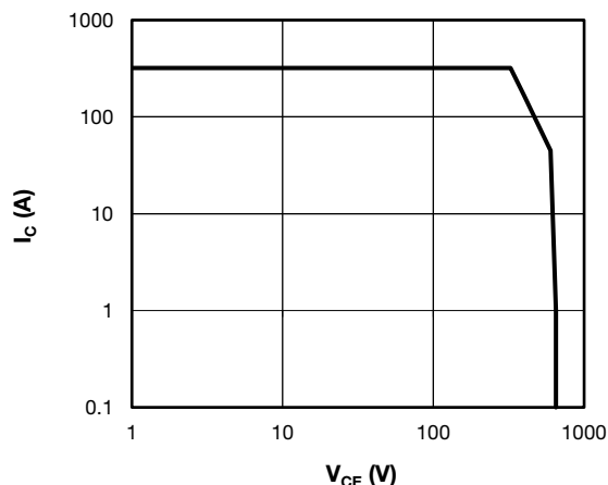
Fig. 17 - Trench IGBT Reverse BIAS SOA T_J = 175^\circ\text{C} , I_C = 320\text{ A} , R_g = 4.7\ \Omega , V_{GE} = +15\text{ V/0 V} , V_{CC} = 325\text{ V} , V_p = 650\text{ V}
