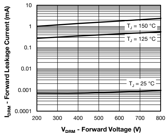
Fig. 6 - Typical Scr1 - Scr2 Forward Leakage Current vs. Direct Blocking Voltage
