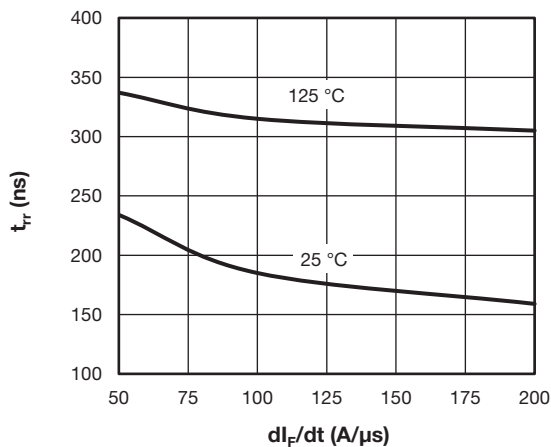
Fig. 6 - Typical Reverse Recovery Time vs. dI_F/dt I_{FM} = 150 A, V_R = 400 V
