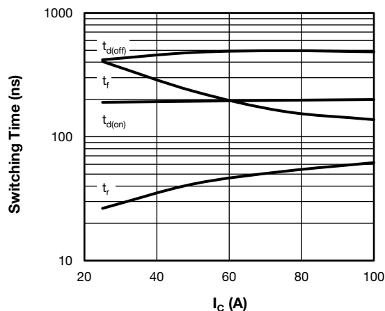
Fig. 12 - Typical IGBT Switching Time vs. I_C T_J = 125\text{ }^{\circ}\text{C} , V_{CC} = 720\text{ V} , R_g = 1.0\text{ }\Omega , V_{GE} = 15\text{ V} , L = 500\text{ }\mu\text{H}
