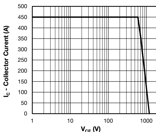
Fig. 21 - IGBT Reverse Bias SOA V_{GE} = 15 \text{ V} , T_J = 150^\circ \text{C}
