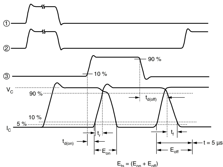
Fig. 25 - Switching Loss Waveforms Test Circuit
