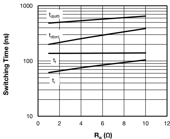
Fig. 14 - Typical IGBT Switching Time vs. R_g T_J = 125\text{ }^{\circ}\text{C} , V_{CC} = 720\text{ V} , I_C = 100\text{ A} , V_{GE} = 15\text{ V} , L = 500\text{ }\mu\text{H}
