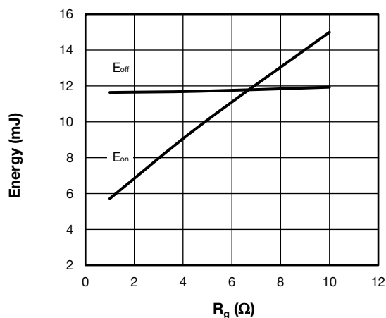
Fig. 13 - Typical IGBT Energy Loss vs. R_g T_J = 125\text{ }^{\circ}\text{C} , V_{CC} = 720\text{ V} , I_C = 100\text{ A} , V_{GE} = 15\text{ V} , L = 500\text{ }\mu\text{H}
