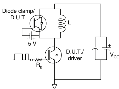
Fig. 24 - Switching Loss Test Circuit
