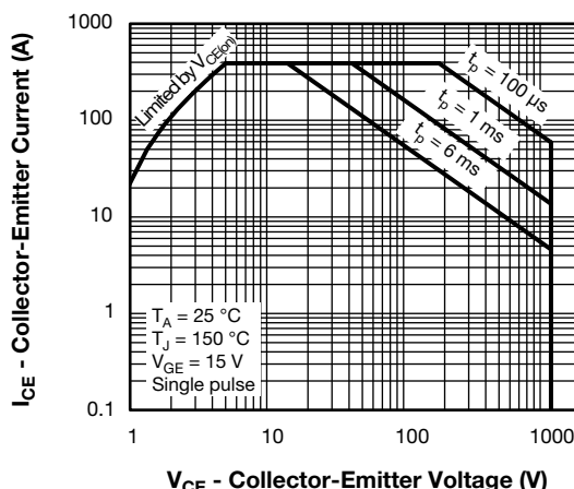
Fig. 18 - IGBT Safe Operating Area
