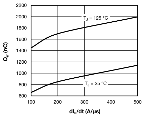
Fig. 17 - Typical Diode Reverse Recovery Charge vs. di_F/dt V_{rr} = 400 \text{ V} , I_F = 50 \text{ A}
