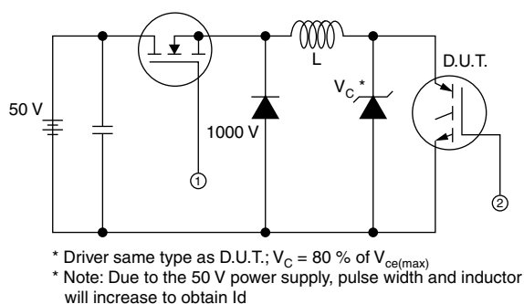
Fig. 22 - Clamped Inductive Load Test Circuit
