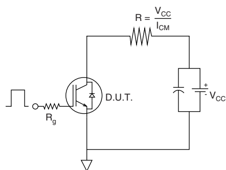
Fig. 23 - Pulsed Collector Current Test Circuit
