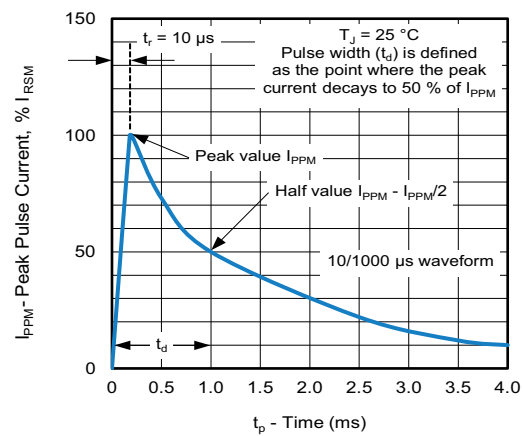
Fig. 4 - Pulse waveform
