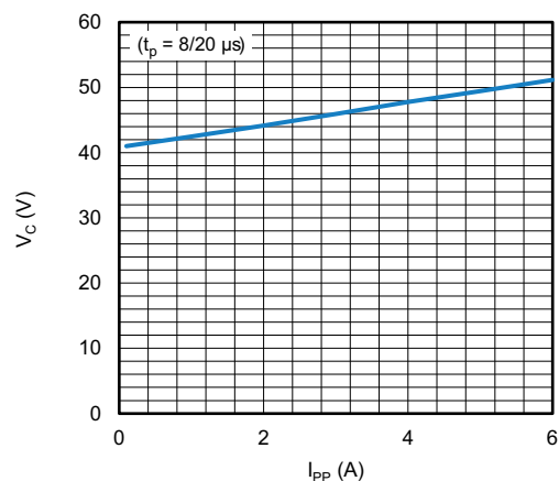
Fig. 6 - Typical Peak Forward Clamping Voltage vs. Peak Pulse Current; t_p = 8/20 \mu s
