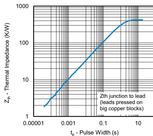
Fig. 10 - Thermal Impedance vs. Time
