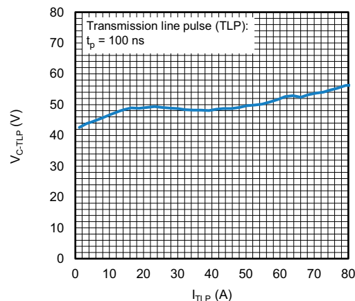
Fig. 8 - Typical Peak Forward Clamping Voltage vs. Peak Pulse Current; t_p = 100 ns (TLP)
