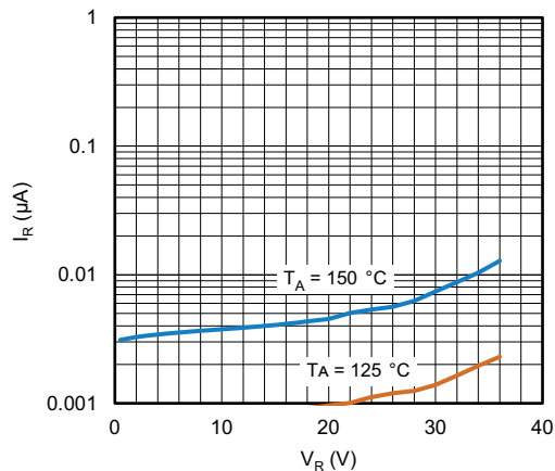
Fig. 5 - Typical Reverse Leakage Current vs. Reverse Voltage
