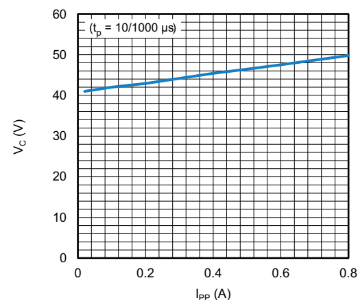
Fig. 7 - Typical Peak Clamping Voltage vs. Peak Pulse Current; t_p = 10/1000 \mu s
