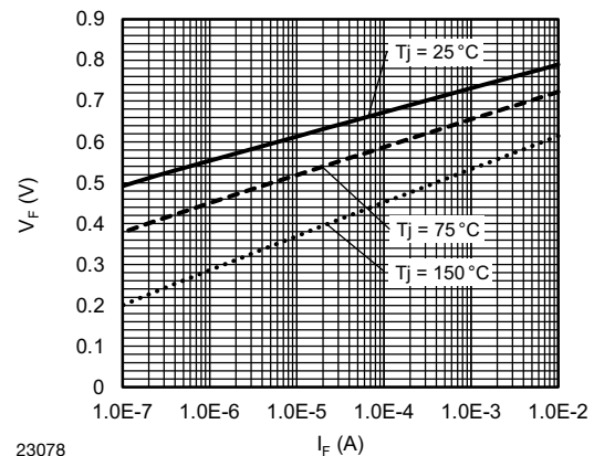
Fig. 6 - Typical Forward Voltage vs. Forward Current
