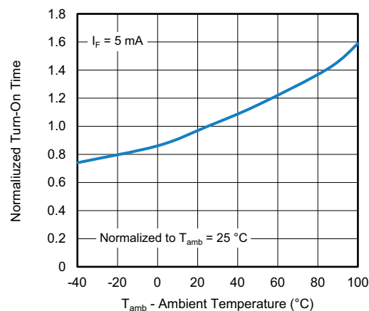
Fig. 12 - Normalized Turn-On Time vs. Ambient Temperature
