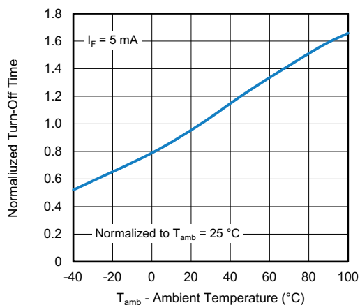
Fig. 14 - Normalized Turn-Off Time vs. Ambient Temperature
