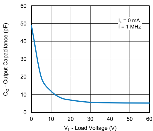
Fig. 9 - Output Capacitance vs. Load Voltage
