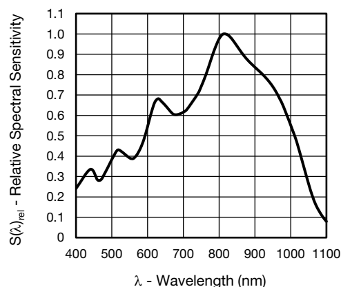
Fig. 2 - Relative Spectral Sensitivity vs. Wavelength without Resin Coating
