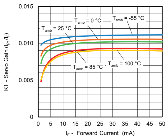
Fig. 6 - Servo Gain vs. Forward Current
