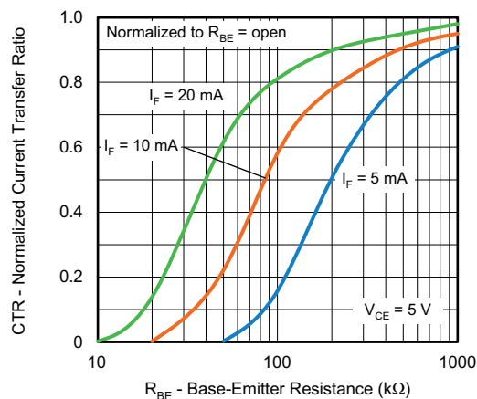
Fig. 5 - Current Transfer Ratio (saturated) vs. Base Emitter Resistance
