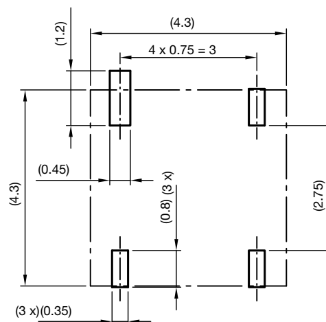
Proposed pad layout from component side (dim. for reference only)
