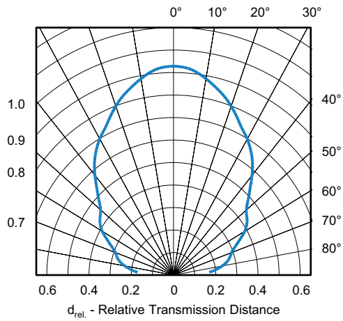
Fig. 11 - Horizontal Directivity
