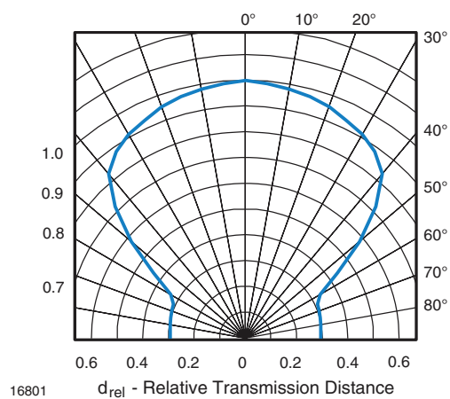
Fig. 11 - Directivity
