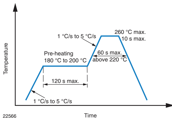
Fig. 9 - Lead (Pb)-Free Reflow Solder Profile According to J-STD-020
