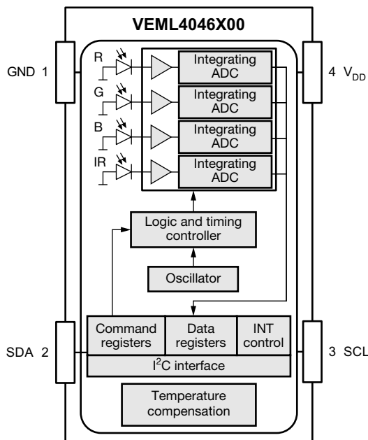
Fig. 1 - Block Diagram
