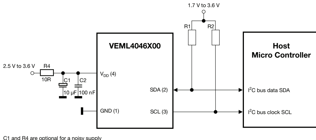
Fig. 9 - Application Circuit (x) = Pin Number
