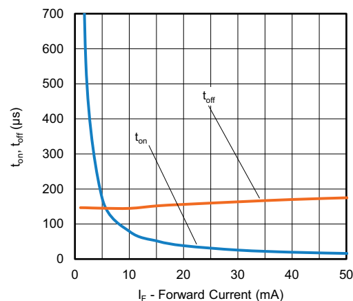
Fig. 5 - t_{on} , t_{off} vs. LED Current
