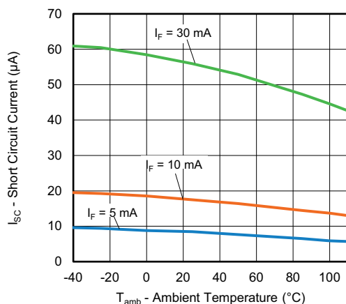
Fig. 3 - Output Short-Circuit Current vs. Ambient Temperature
