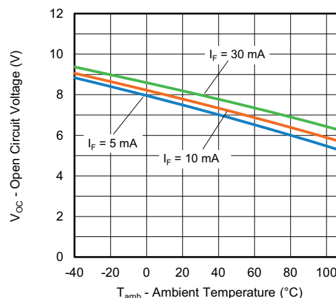
Fig. 4 - Output Open Circuit Voltage vs. Ambient Temperature
