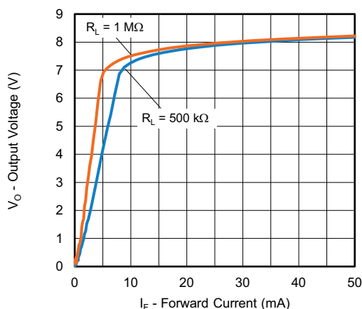
Fig. 2 - Output Open Circuit Voltage vs. LED Current
