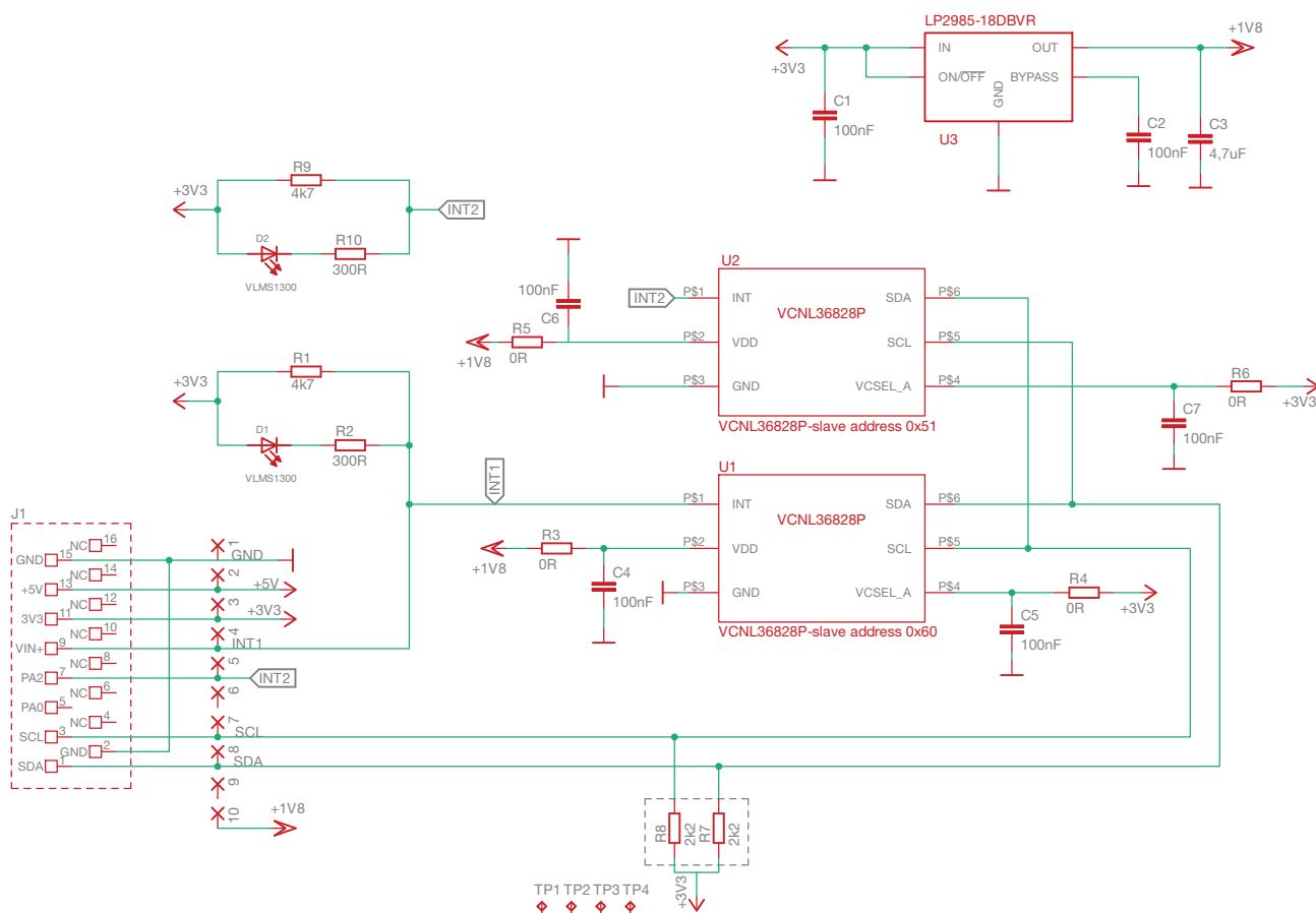
Fig. 4 - Schematic of the VCNL36828P Sensor Board
