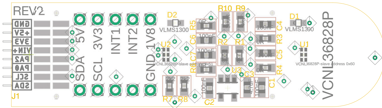
Assembly top
