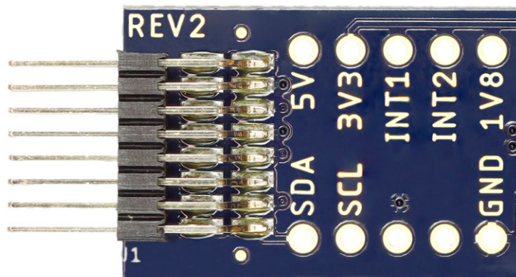
Fig. 3 - Connection of the Sensor Board (power supply and I 2 C lines)
