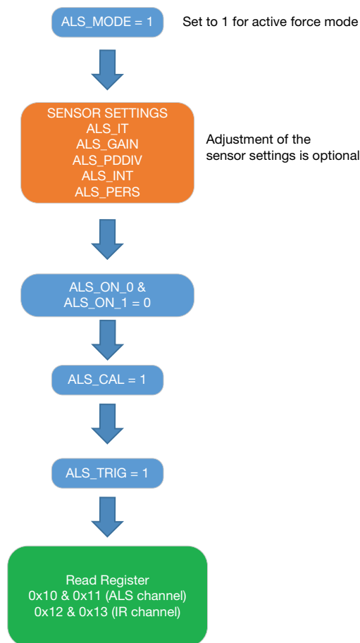
Fig. 5 - Basic Initialization for Active Force Mode
