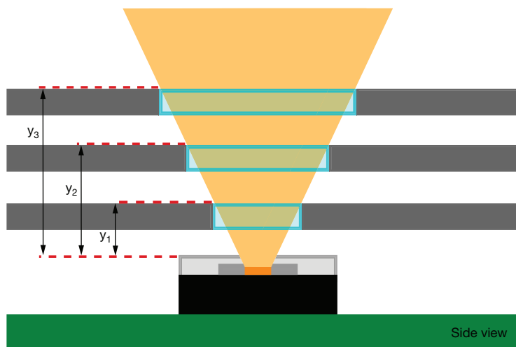
Fig. 15 - Asymmetric Window Design Where the Diameter Increases With Increasing Distance From the Sensor
