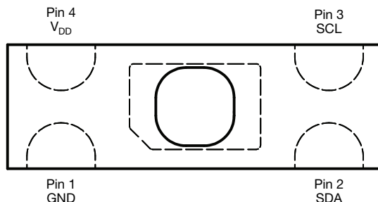
Fig. 1 - Pin Assignment (Top View) of the VEML4031X00
