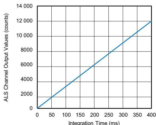
Fig. 11 - Linearity of the Integration Time
