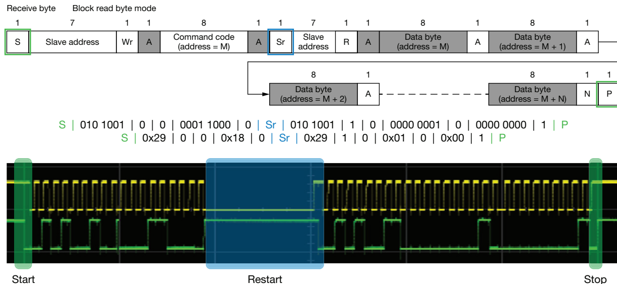
Fig. 8 - I 2 C Read With Necessary Repeated Start Condition
