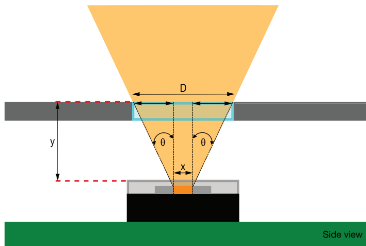
Fig. 17 - Window Design Calculation
