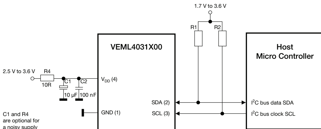
Fig. 3 - Application Circuitry to Communicate With the VEML4031X00 via I²C
