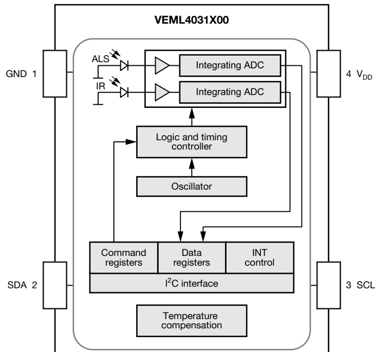
Fig. 2 - Block Diagram
