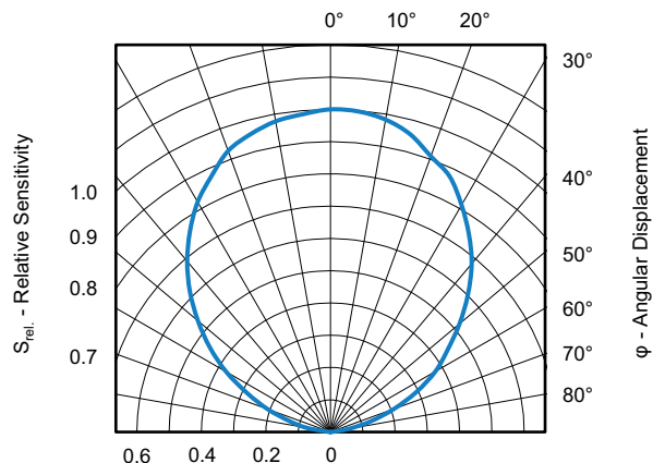
Fig. 16 - Relative Sensitivity vs. Angular Displacement
