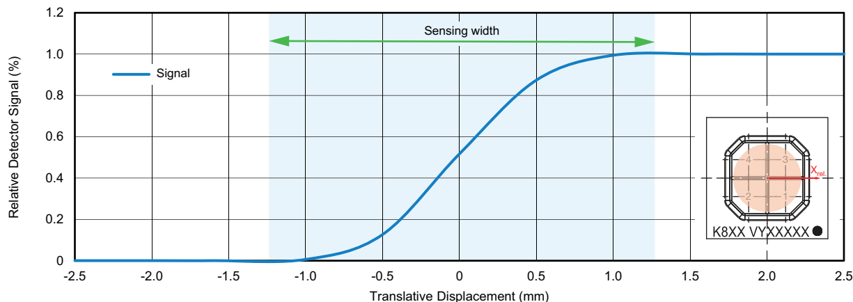
Fig. 2 - Relative Output Signal vs. Translative Displacements X_{rel.} of the Light Spot (Light Spot Diameter: b = 1.5 mm)
