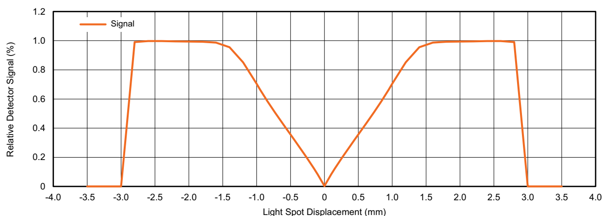
Fig. 4 - M-Shaped Signal Response vs. Translative Light Spot Displacement
