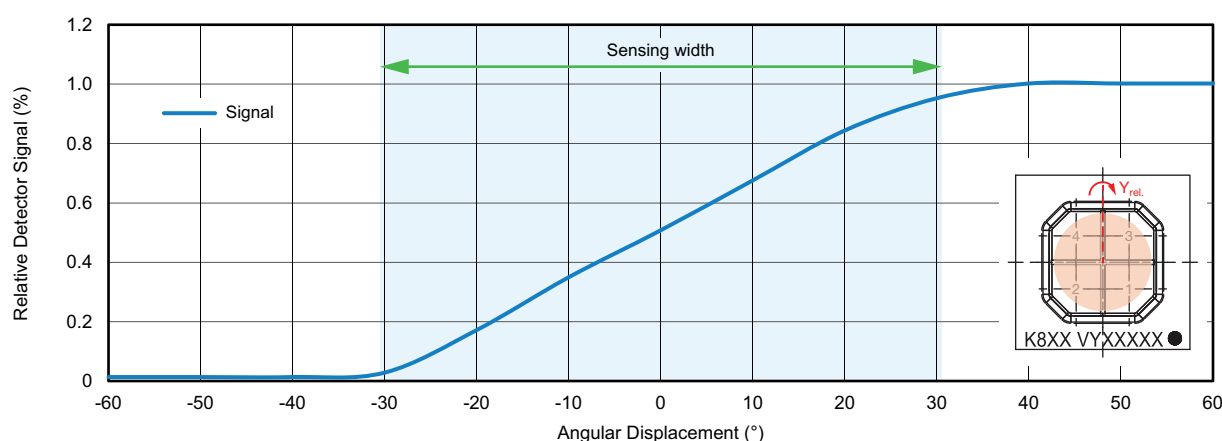
Fig. 3 - Relative Output Signal vs. Angular Displacement Y_{rel.} of the Light Spot (Aperture Dimensions: a = 3.0 ; t = 1.0 ; d = 1.0 )
