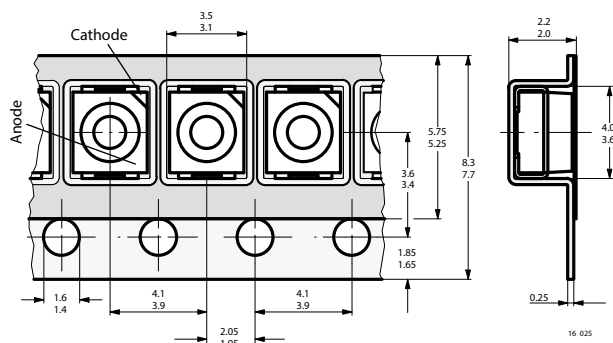
Fig. 9 - Tape Dimensions in mm for PLCC-2
