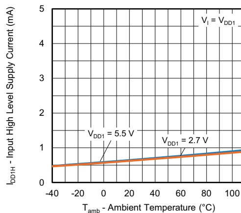
Fig. 8 - Input High Level Supply Current vs. Ambient Temperature
