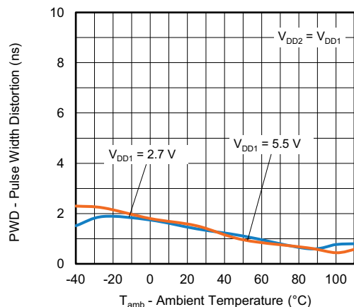
Fig. 17 - Pulse Width Distortion vs. Ambient Temperature
