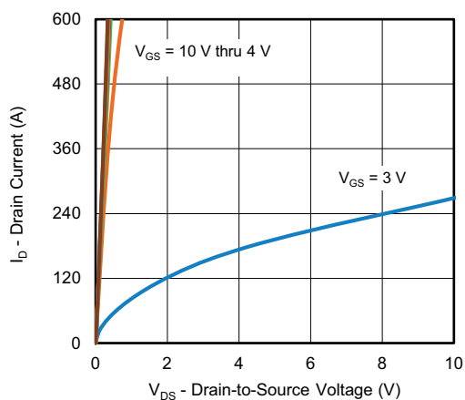
Fig. 1 - Output Characteristics
