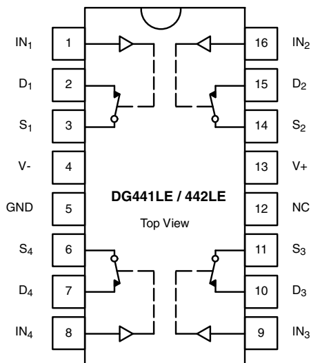
Dual-In-Line, TSSOP and SOIC
