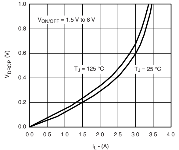
V_{DROP} vs. I_L at V_{IN} = 1.8\text{ V}
