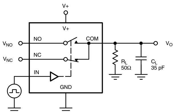
Fig. 1 - Switching Time
