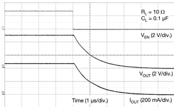
Fig. 24 - Turn-Off (V IN = 5 V)
