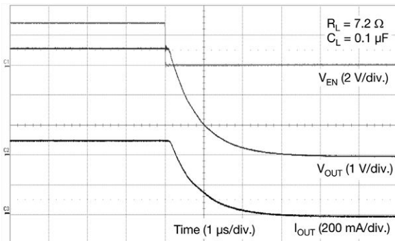
Fig. 23 - Turn-Off (V IN = 3.6 V)
