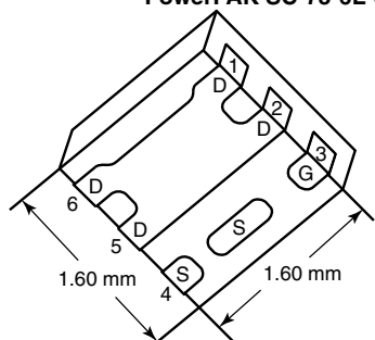
PowerPAK SC-75-6L-Single
