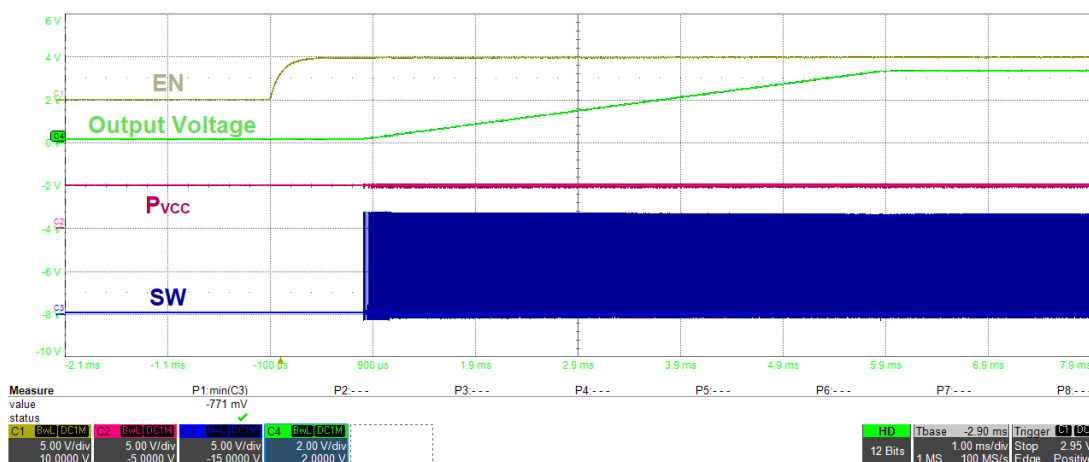
Fig. 14 - Startup with EN, 12 A Load (5 ms/div)
