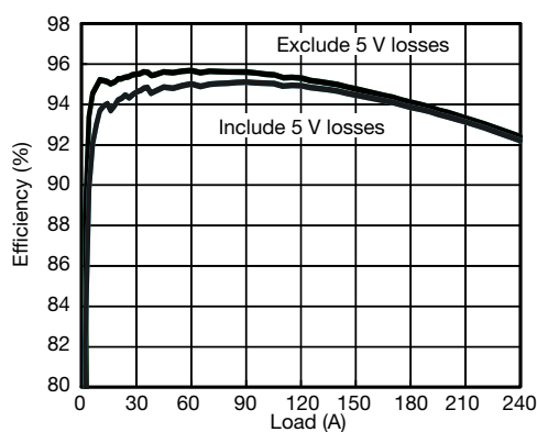
Fig. 5 - 1.8 V V_{OUT} Power Stage Efficiency ( V_{IN} = 12 V, f_{SW} = 500 kHz; L_{OUT} = 0.18 \mu H/0.17m \Omega /FP1008-180-R; Auto-Phase Enabled in 6-Phase Operation)
