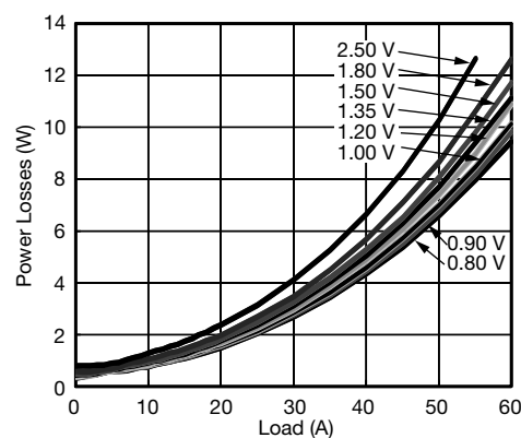
Fig. 7 - Power Dissipation ( V_{IN} = 12\text{ V} , f_{SW} = 500\text{ kHz} ; L_{OUT} = 0.18\text{ }\mu\text{H}/0.17\text{ m}\Omega/\text{FP1008-180-R} )
