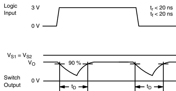
Fig. 3 - Break-Before-Make (DG419)
