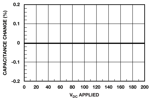
C0G (NP0)/(CG)
