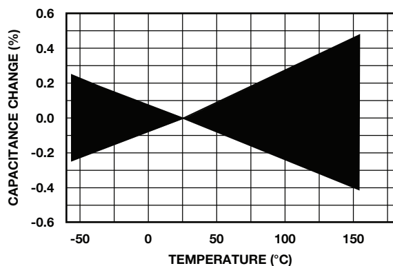
C0G (NP0)/(CG)
