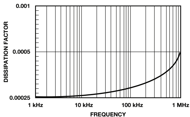
C0G (NP0)/(CG)
