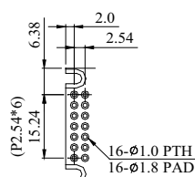
PIN DETAIL
