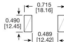
Typical Pad Layout
