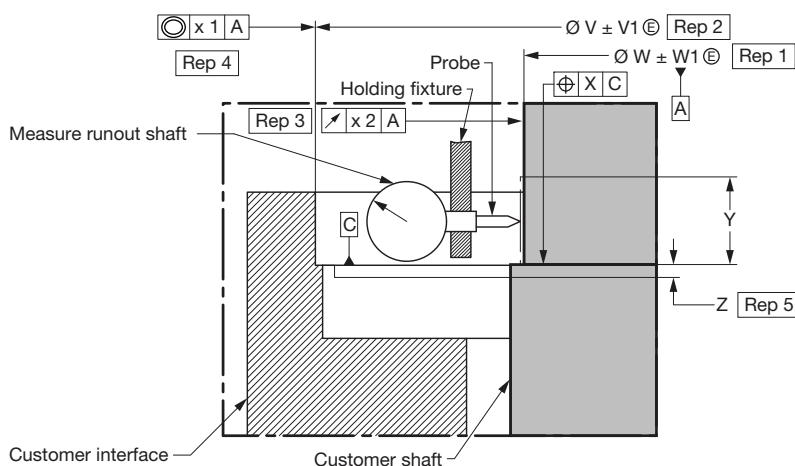
Fig. 1 - Mounting Detail
