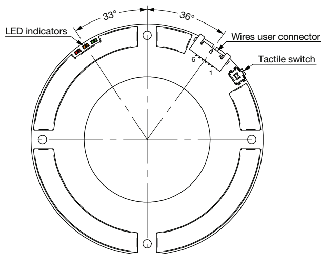
Fig. 6 - User Connector
