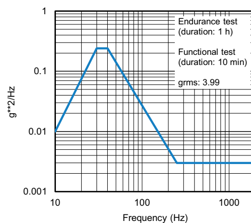
Fig. 3 - Vibration Profile 4
