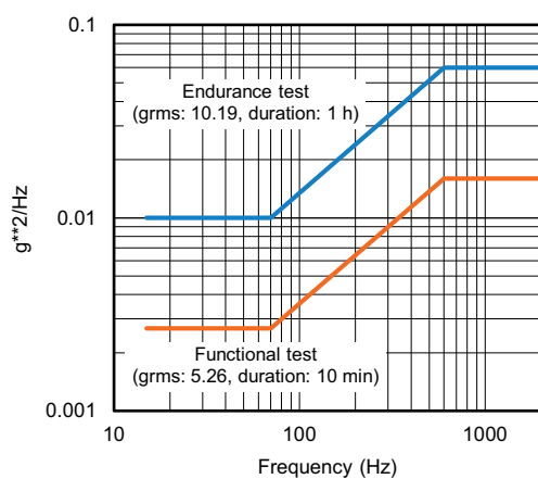
Fig. 2 - Vibration Profile 3
