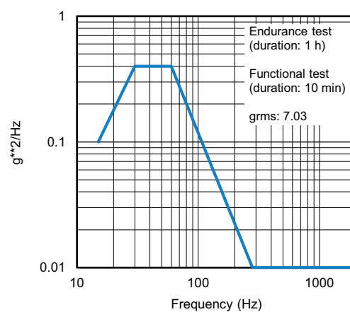
Fig. 4 - Vibration Profile 5
