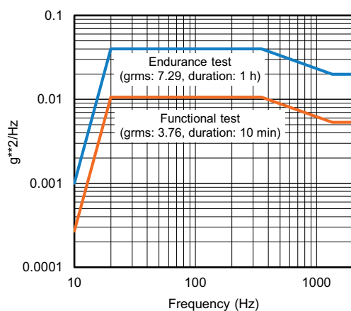
Fig. 1 - Vibration Profile 2
