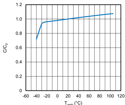
Fig. 5 - Typical multiplier of capacitance as a function of ambient temperature ( C_0 = typical capacitance at 20 °C, 100 Hz)
