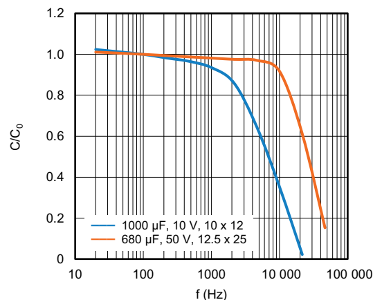
Fig. 6 - Typical multiplier of capacitance as a function of frequency ( C_0 = typical capacitance at 20 °C, 100 Hz; T_{amb} = 20 °C)
