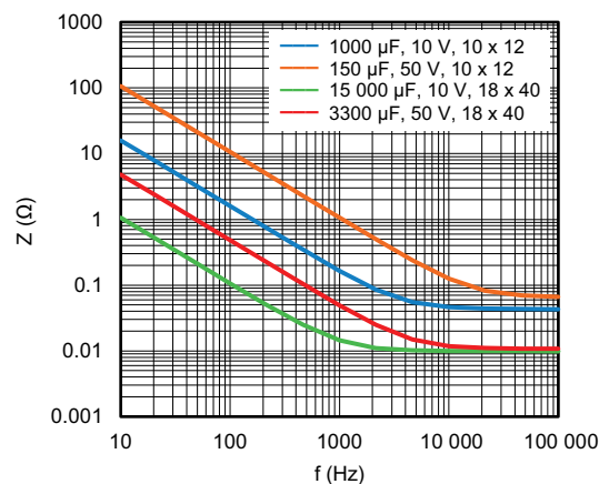
Fig. 10 - Typical impedance as a function of frequency ( T_{amb} = 20 °C)
