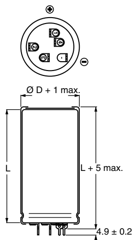
Fig. 4 - Printed wiring pin version (Case \varnothing D = 40 mm)
