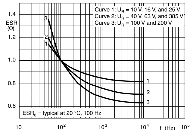
Fig. 12 - Typical multiplier of typical ESR as a function of frequency
