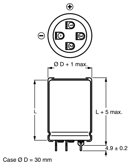
Fig. 4 - Printed wiring pin version
