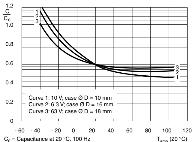
Fig. 7 - Typical multiplier of ESR
