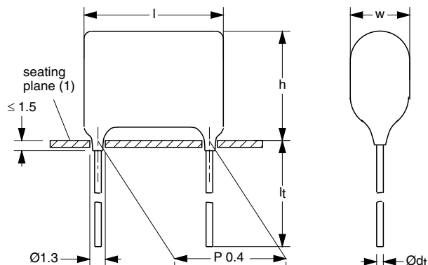
Dimensions in mm (1) Hole Ø 1.0 for d_t = 0.6 mm
