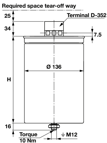
Drawing 1
