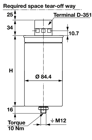
Drawing 3
